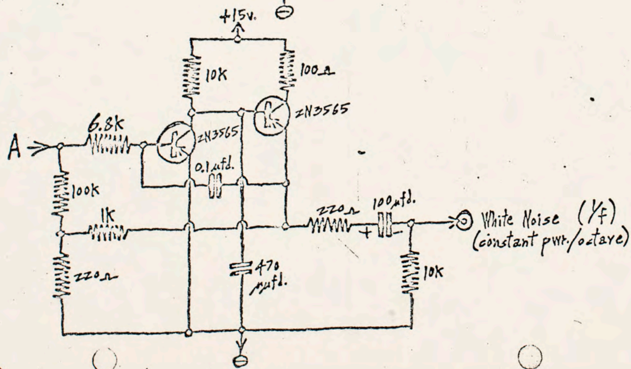
Buchla White Noise Generator (Model 160)
