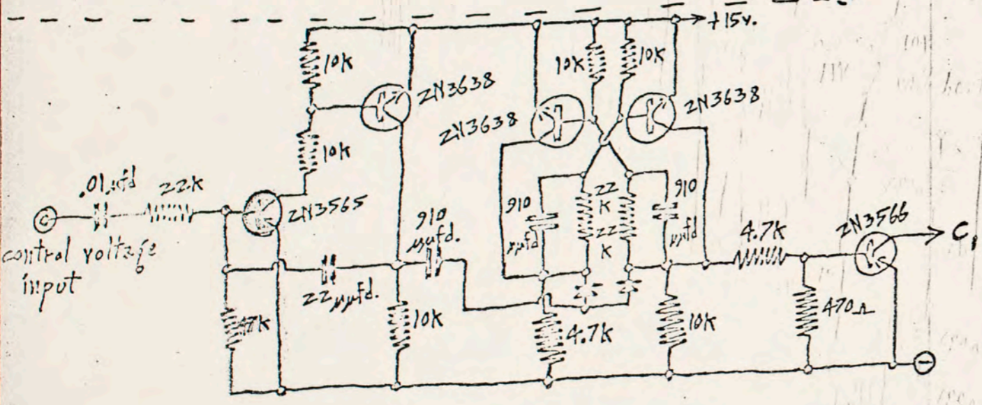
Buchtz Random Voltage Source (Model 165)
